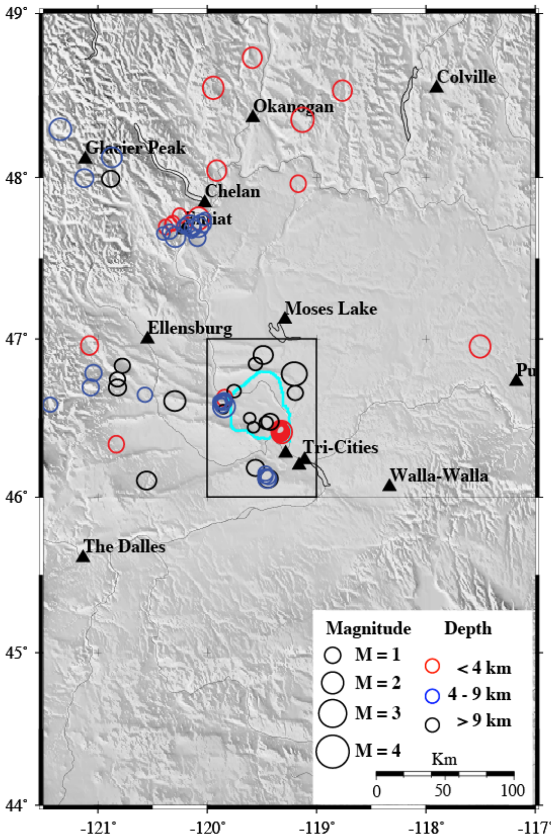
Figure 4.1 Epicenters of earthquakes recorded in the Eastern Washington region during the 2 nd Quarter of FY2014. Black triangles show locations of cities, towns, and volcanoes. Light blue line is the outline of the Hanford site. Black rectangle outlines area mapped in Figure 4.2. Circles are earthquake epicenters, with size scaled by magnitude [radius (in inches) = 0.05*M + 0.1]. Representative symbols for magnitudes 1-4 are shown in the legend. Epicenter symbols are colored by depth, as shown in legend.
