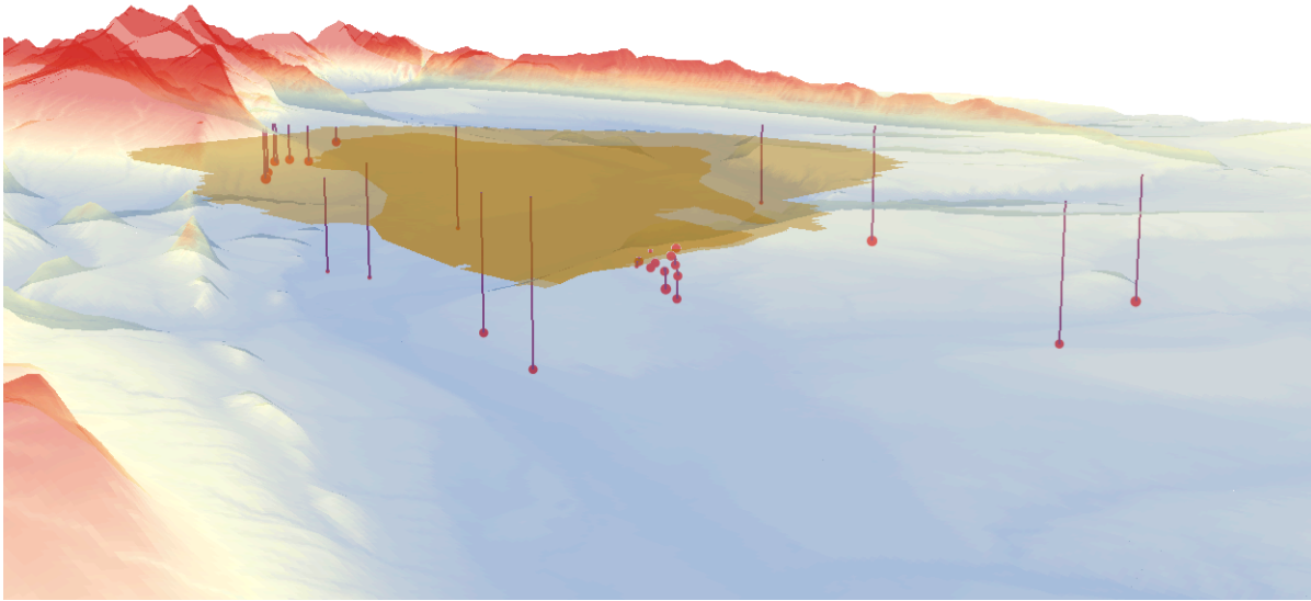
Figure 4.3 Perspective plot showing topography (exaggerated) and hypocenters (red dots, connected to epicenter with fine vertical line) of earthquakes occurring during the 2 nd Quarter of FY2014 in the vicinity of the Hanford site, both overall (lightly shaded region), and inner (darker shading). Probable blasts are not shown in this figure.
