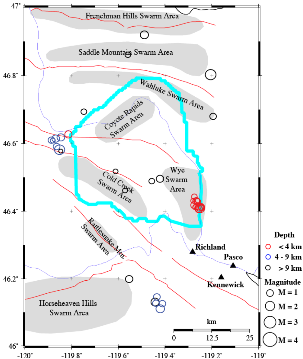
Figure 4.2 Epicenters of earthquakes occurring during the 2 nd Quarter of FY2014 in the vicinity of the Hanford site (blue outline), and their relationship to known structures (red lines), swarm areas (shaded regions), and cultural features and cities (black triangles). Circles are earthquake epicenters, with size scaled by magnitude [radius (in inches) = 0.05 * M + 0.1 ]. Representative symbols for magnitudes 1-4 are shown in the legend. Epicenter symbols are colored by depth, as shown in legend.
