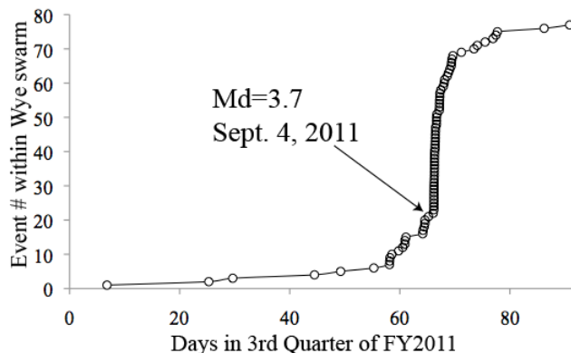
Wye Swarm Earthquakes, July-Sept. 2011
