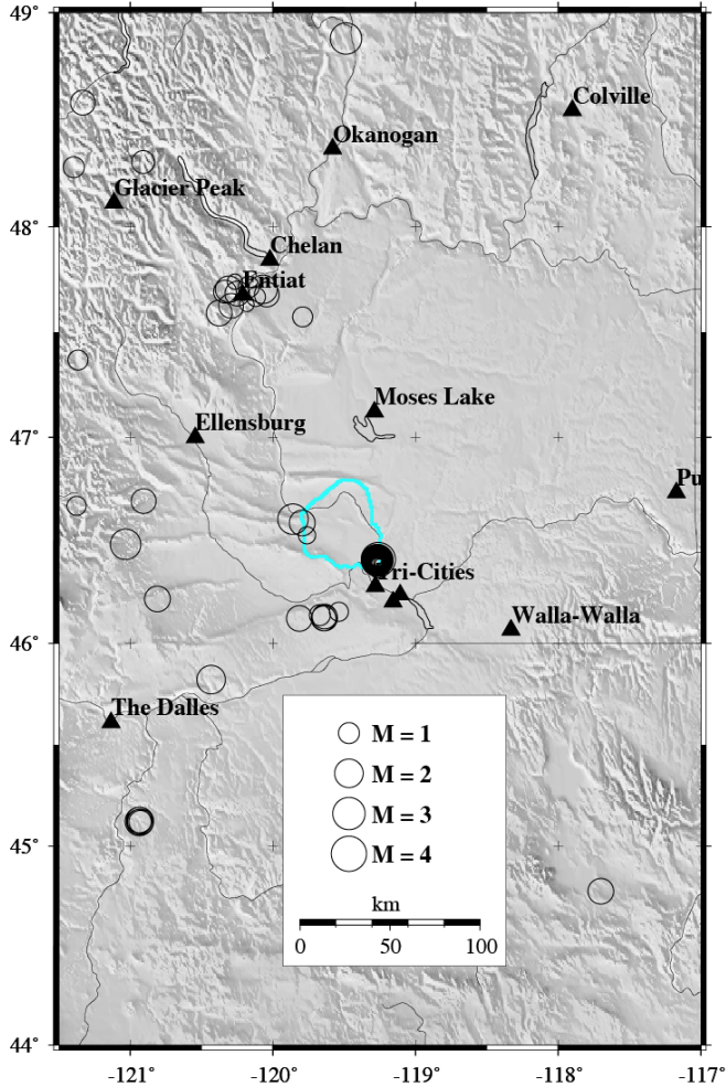
Figure 5.2 Epicenters of earthquakes recorded in the wider Hanford area during the 4 th Quarter of 2011.
