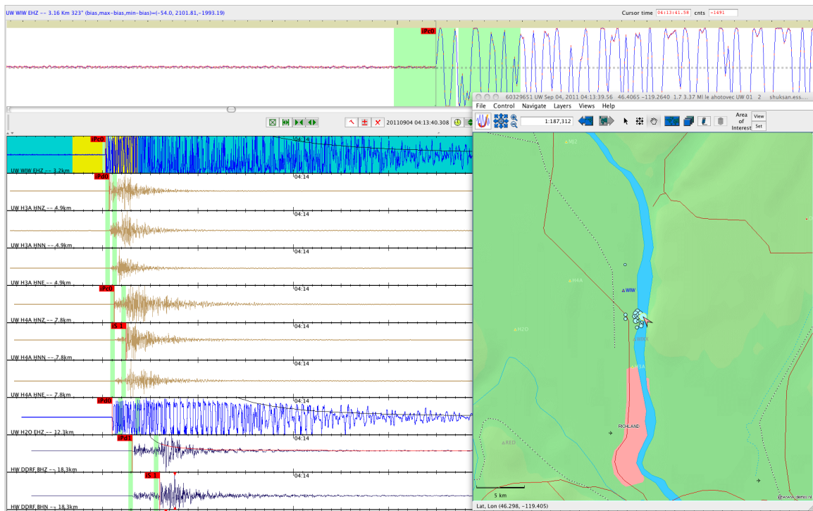
Figure 6.1 Screen shot of analyst’s view of the data from the 4 September, 2011 M_d 3.7 Wooded Island swarm earthquake. Note the clipped seismograms from the high-gain analog station (blue traces), and the data from the strong motion stations H3A and H4A (brown traces). Red label “flags” attached to thin red bars reveal time of analyst-reviewed phase picks, labeled with pick type and weight.
