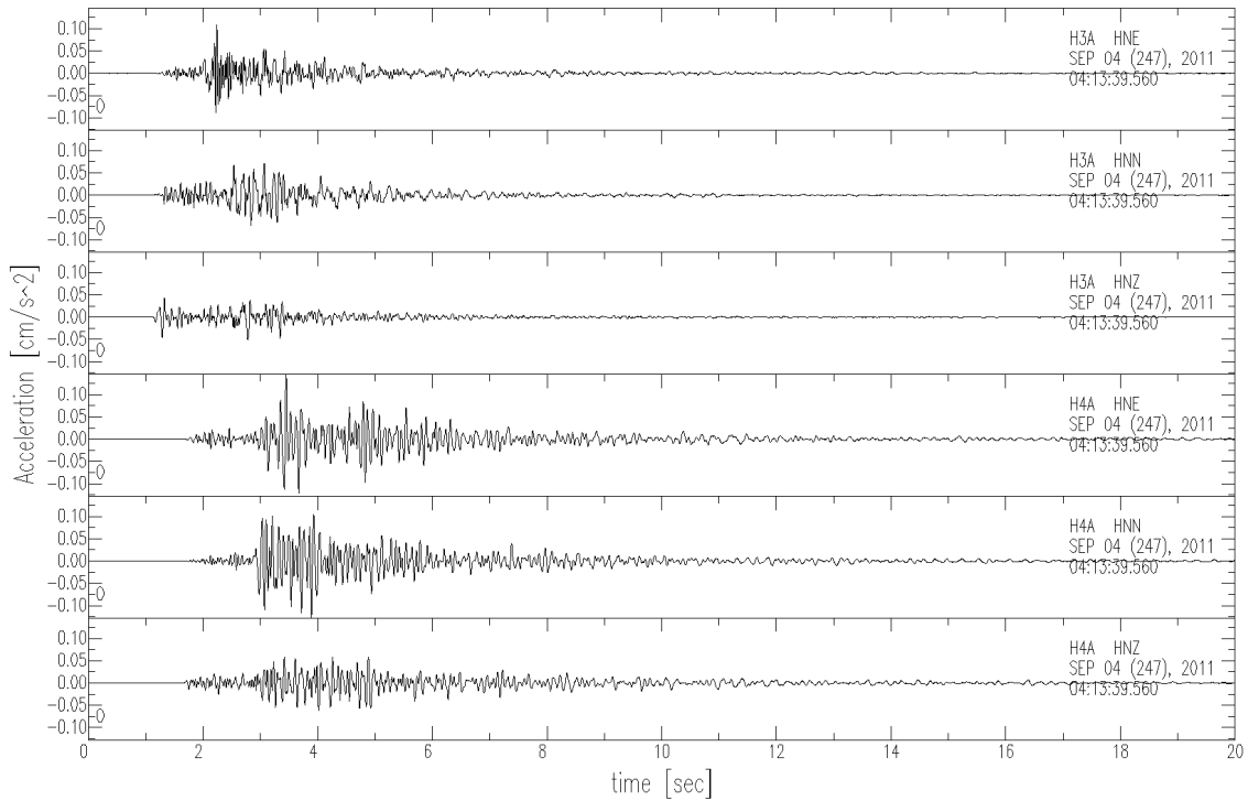
Figure 6.2 Instrument-corrected ground motions from the 4 September, 2011, M_d 3.7 earthquake, recorded at H3A (top 3 traces) and H4A (Bottom 3 traces). For each station, the top waveform is the east component, the next panel is the north component and the bottom waveform shows vertical ground accelerations. These records verify that shaking levels were not close to levels that might be expected to cause damage, but of a level sufficient to be felt rather sharply.
