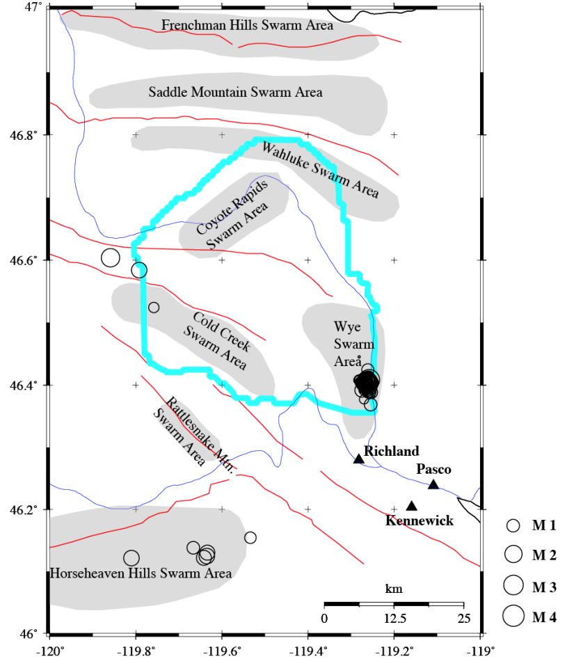
Figure 5.3 Epicenters of earthquakes occurring during the 4 th Quarter of 2011 in the vicinity of the Hanford site (blue outline), and their relationship to known structures (red lines), swarm areas (shaded bits), and cultural features.
