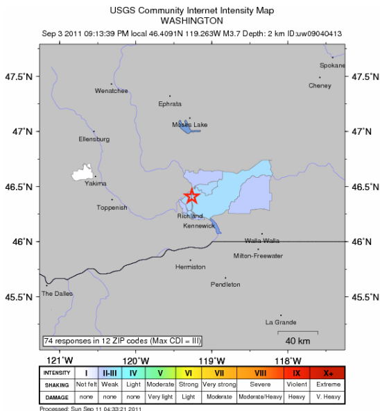
Figure 6.3 Community Internet Intensity map. This figure shows Internet-gathered reports of felt shaking intensities self-reported from the local community for the 4 September, 2011 M 3.7 Wye swarm (Wooded Island) earthquake.
